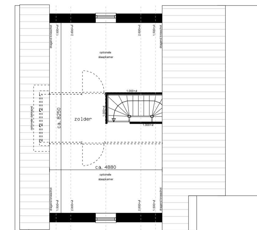
ZOLDER 5.800+P
